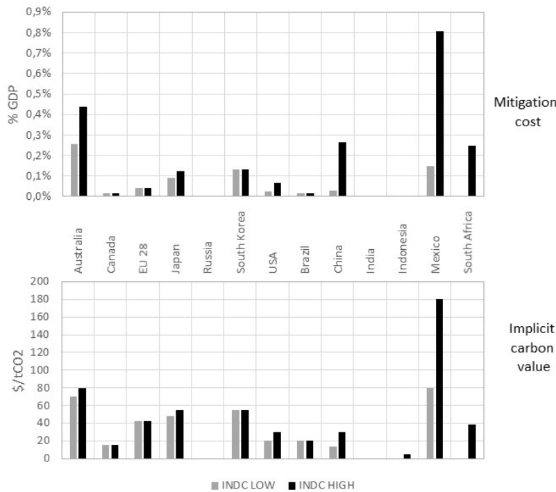
Figure 4: Implicit carbon values and mitigation cost (/GDP) for DDPP countries in NDC scenarios in 2030
