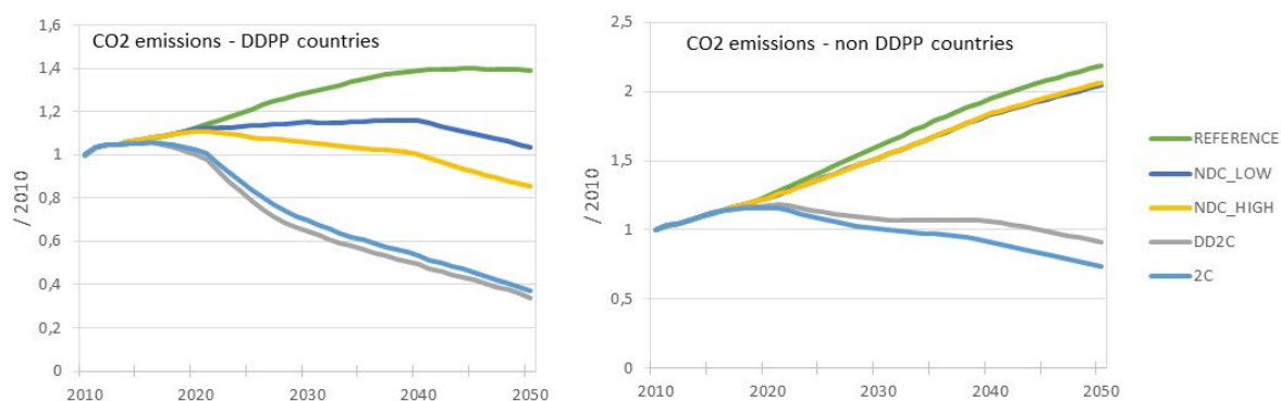
Figure 1: Global energy-related CO 2 emissions in DDPP and non-DDPP countries
