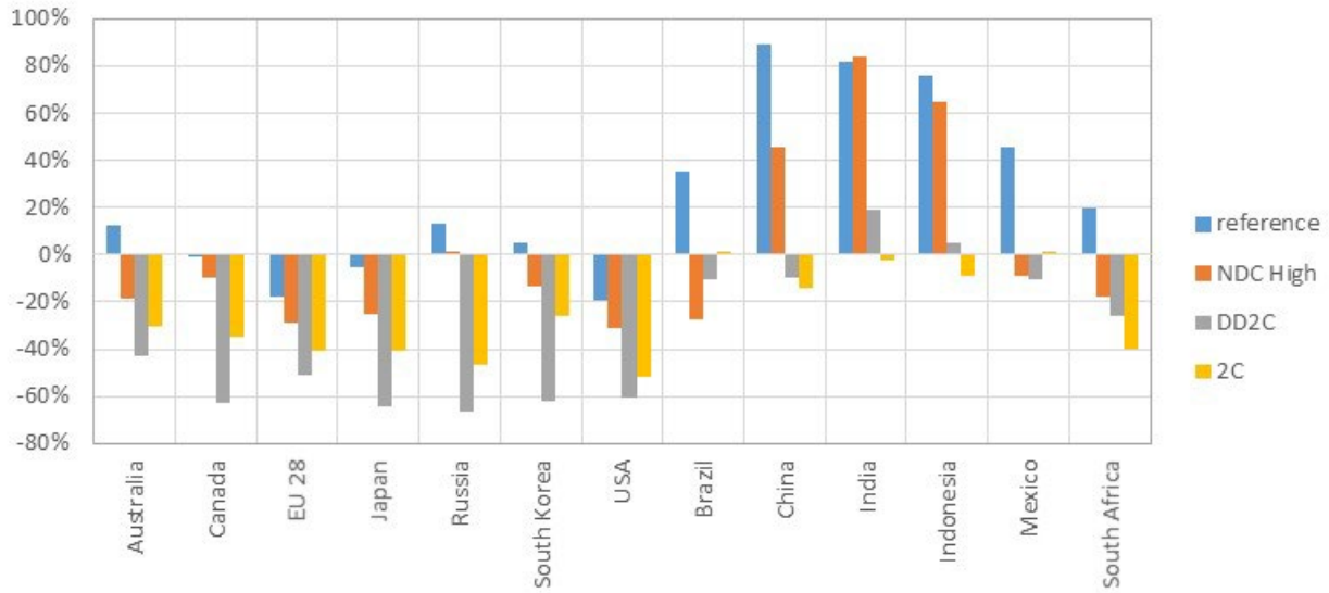
Figure 2: CO2 energy-related emissions in 2030 with respect to 2010 in the reference scenario and in mitigation scenarios for the DDPP countries
