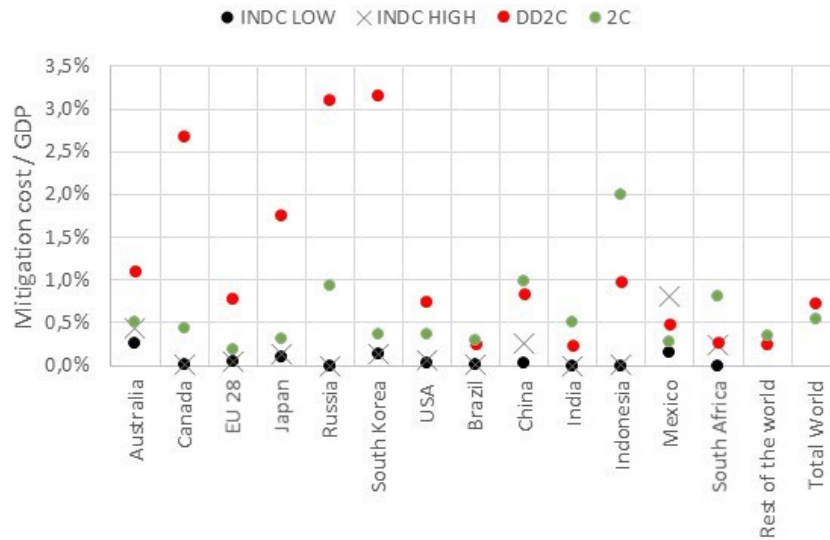
Figure 6: National mitigation cost (/GDP) in mitigation scenarios
