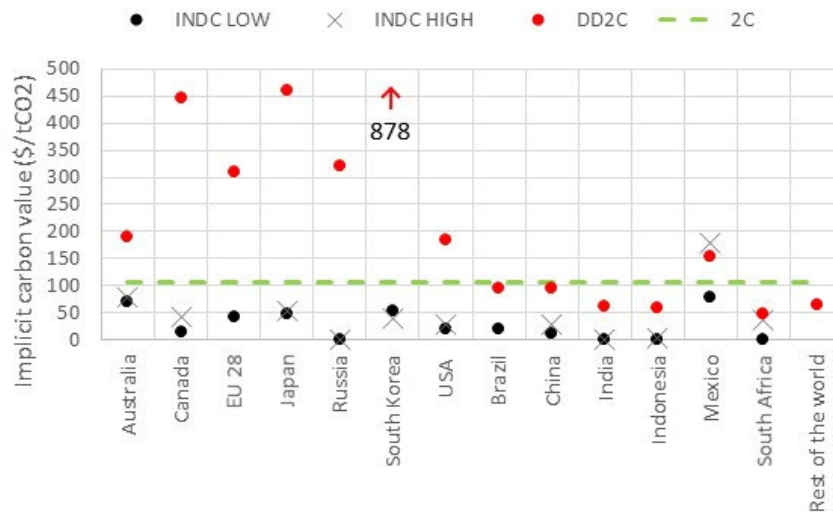
Figure 5: Implicit carbon values in mitigation scenarios in 2030
