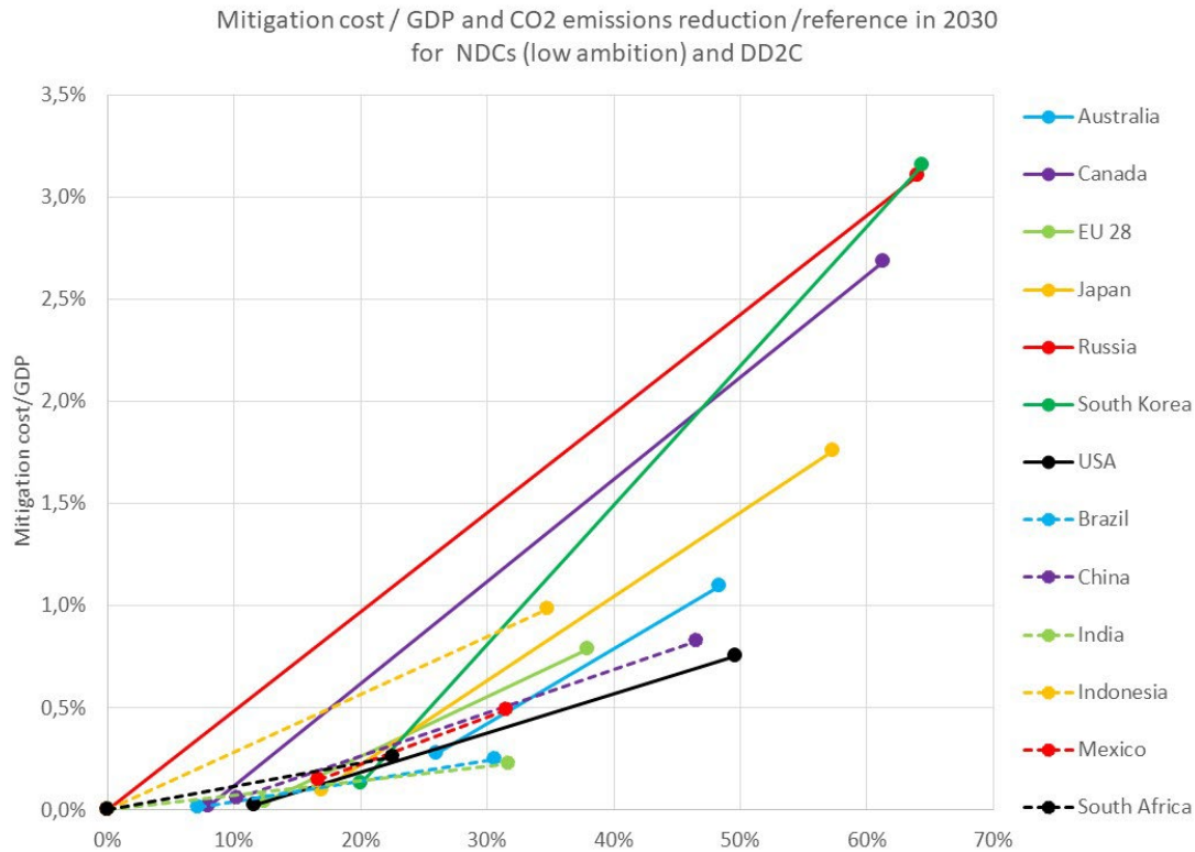
Figure 8: National mitigation cost (/GDP) and energy-related CO 2 emissions abatement compared to the reference scenario in 2030 for NDC LOW and DD2C
