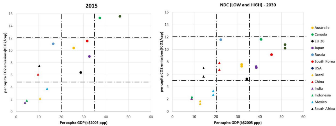
Figure 3: CO2 energy-related emissions per capita (for DDPP countries) plotted against per capita GDP in 2015 and in 2030 for NDC LOW NDC HIGH, DD2C and 2C scenarios
