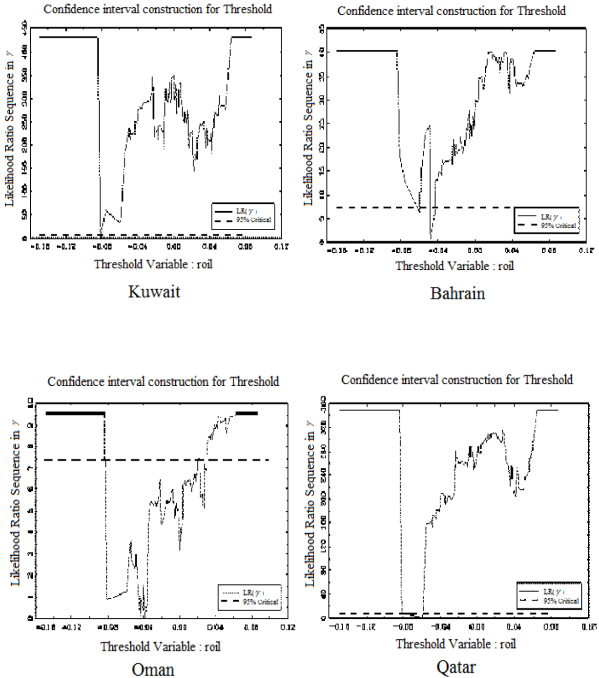
Figure 1: Confidence Interval Construction for Threshold
